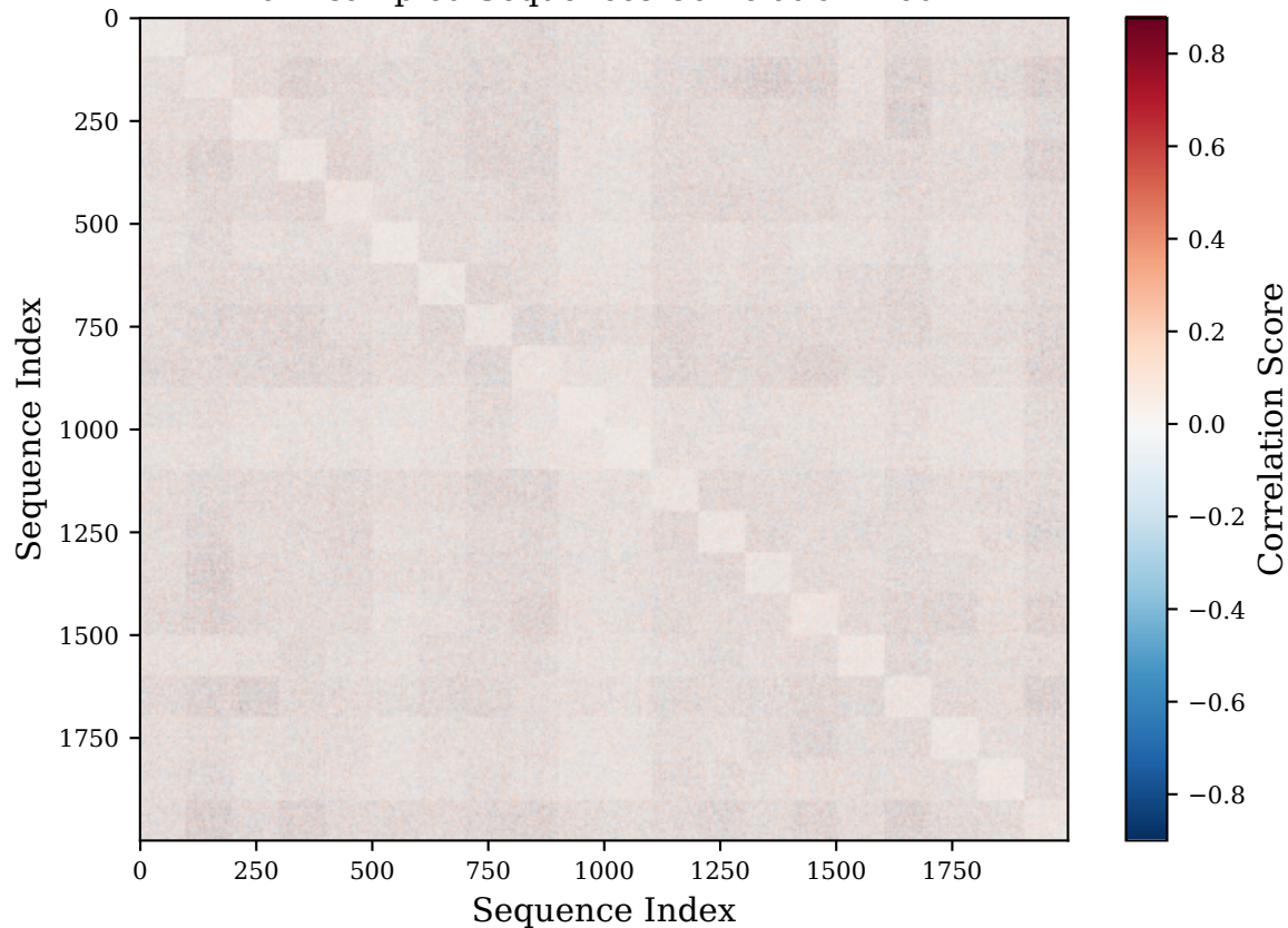
Downsampled Sequences Correlation Matrix
